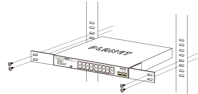
Figure 5-2: Mounting the 802.3at PoE+ Switch in a Rack
