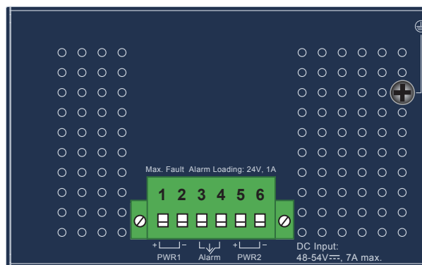
Figure 2-3: IGS-1020PTF Upper Panel
