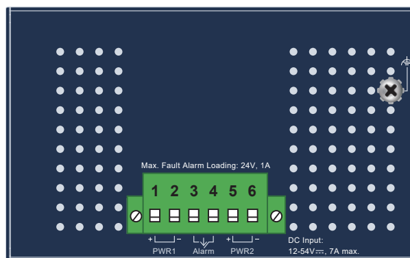
Figure 2-4: IGS-1020PTF-12V Upper Panel
