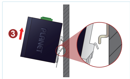
DIN-rail Mounting Installation
