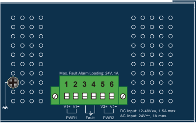
Figure 2: IGS-1600T Top View
