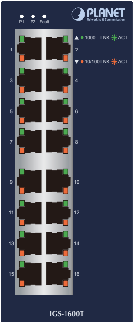
Figure 1: IGS-1600T Front View
