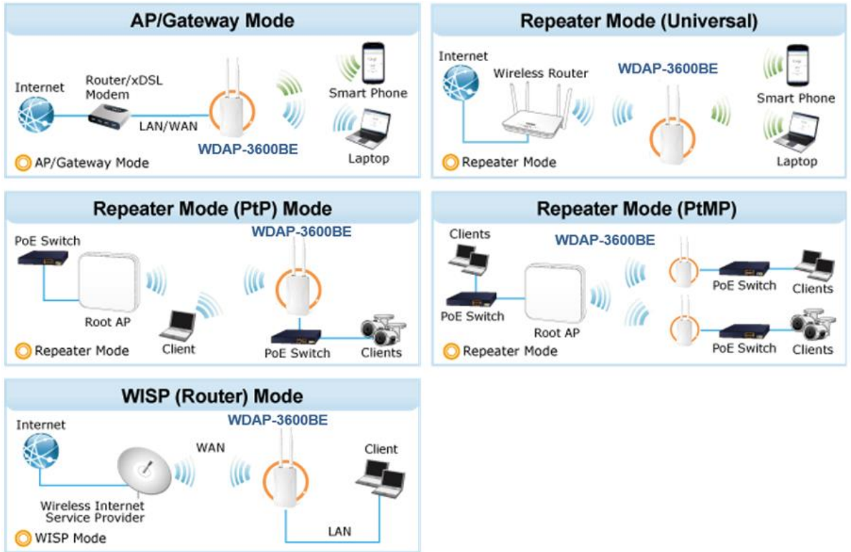
Figure 4-5 Operation Mode
