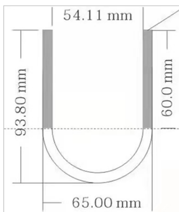
U-bolt Dimensions
