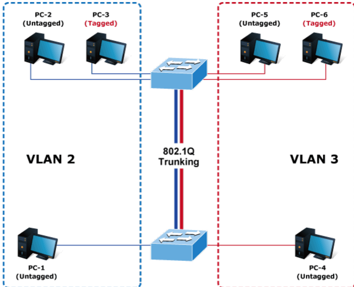
Figure 4-3-56 VLAN Trunking between two 802.1Q aware switches
