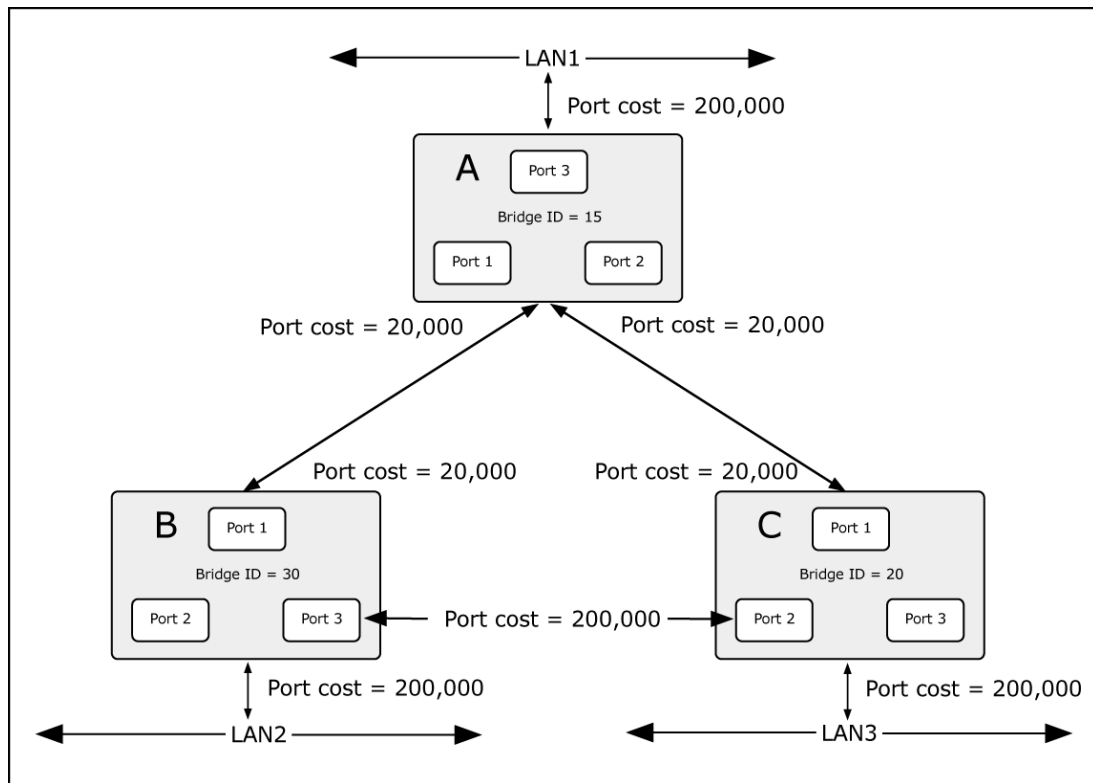
Figure 4-3-58 Before Applying the STA Rules
