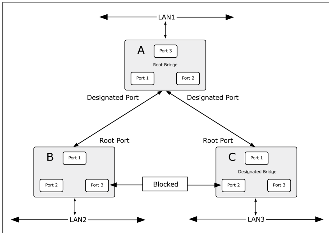
Figure 4-3-59 After Applying the STA Rules
