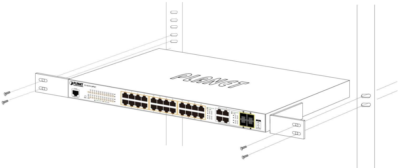
Figure 2-1-6 Mounting Managed Switch in a Rack
