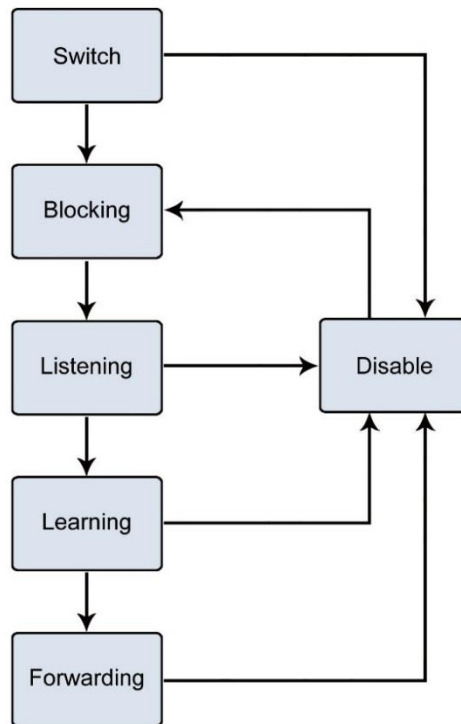
Figure 4-3-57 STP Port State Transitions
