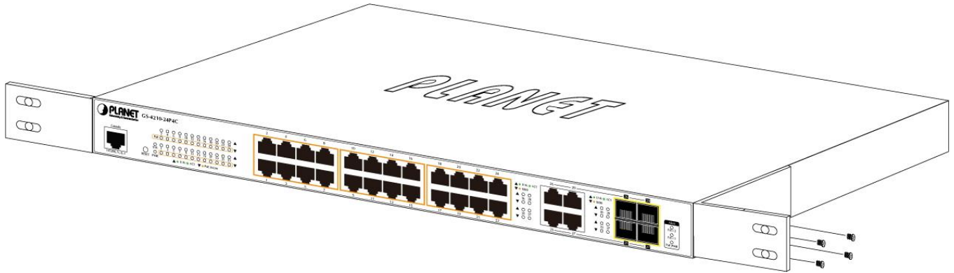
Figure 2-1-5 Attach Brackets to the Managed Switch.
