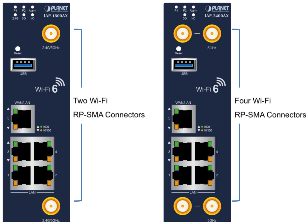
Figure 2-2: Industrial 802.11ax Wireless AP Front Panels
