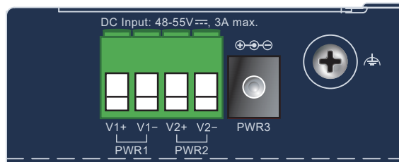
Figure 3: ISW-504PT-E Top View
