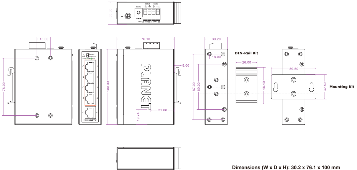
Figure 1: ISW-504PT-E Three-View Diagram
