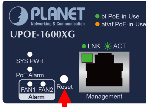
Figure 2-1-4: Reset Button of 10Gbps 802.3bt PoE++ Managed Injector Hub
